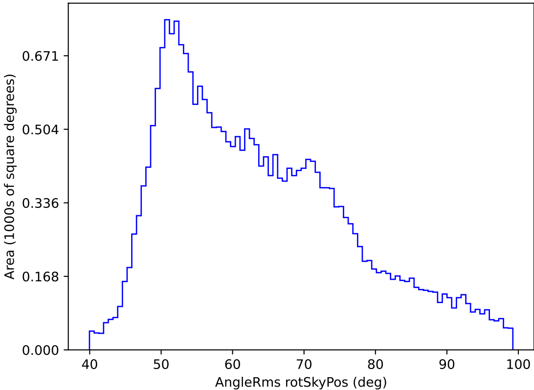
weather_cloudso36v3.4_10yrs All sky r band: AngleRms rotSkyPos
