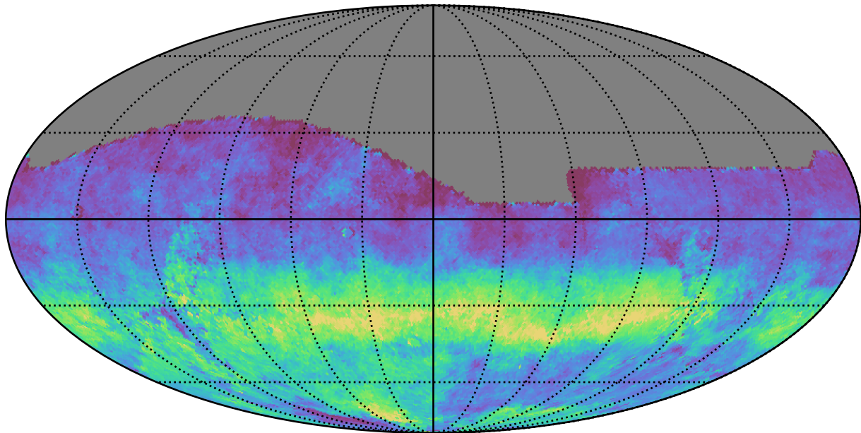
weather_cloudso36v3.4_10yrs All sky g band: AngleRms rotSkyPos
