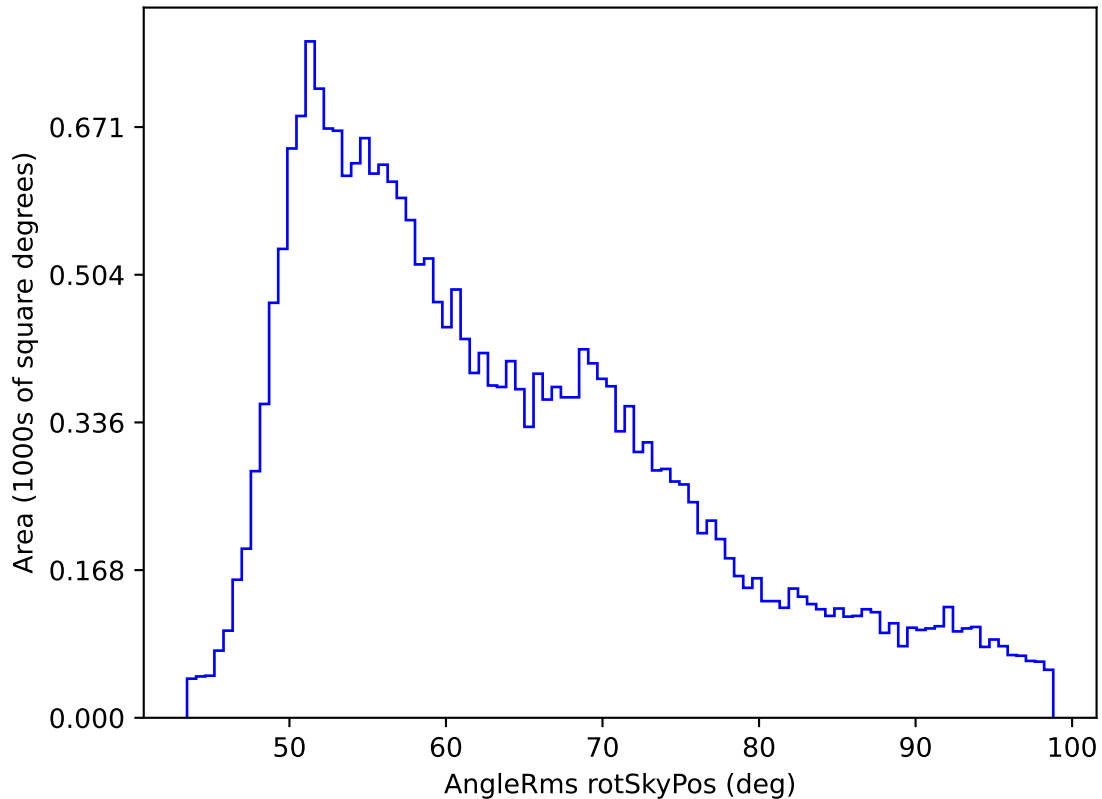
weather_cloudso36v3.4_10yrs All sky all bands: AngleRms rotSkyPos
