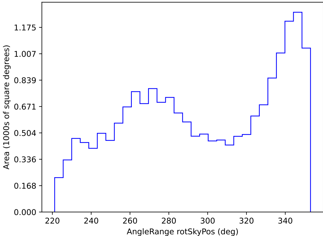
weather_cloudso36v3.4_10yrs WFD all bands: AngleRange rotSkyPos
