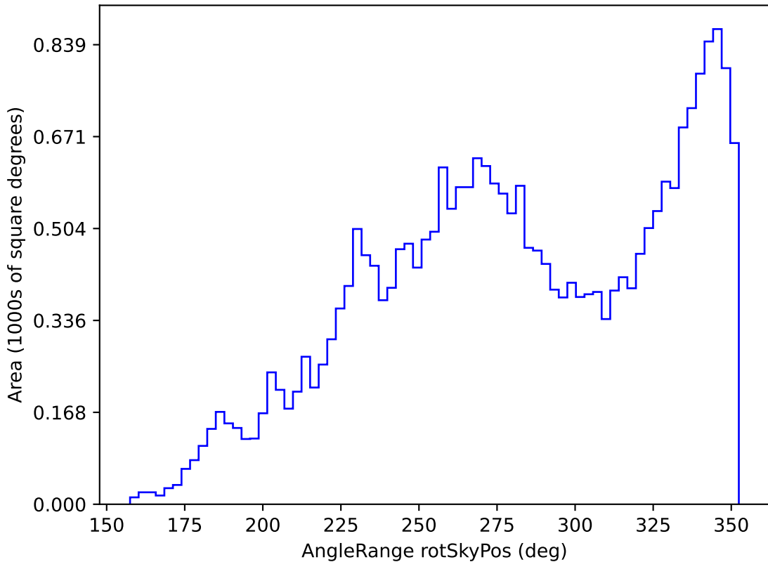
weather_cloudso36v3.4_10yrs All sky all bands: AngleRange rotSkyPos
