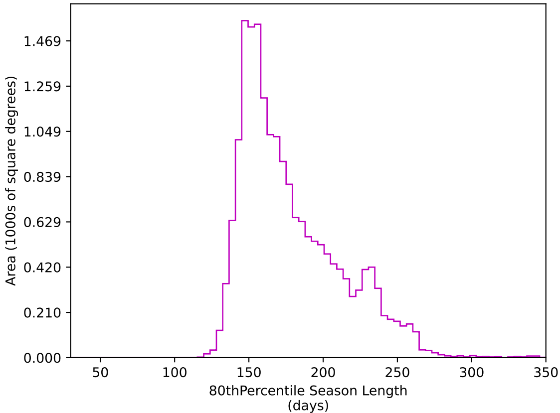
weather_cloudso36v3.4_10yrs WFD z band: 80thPercentile Season Length
