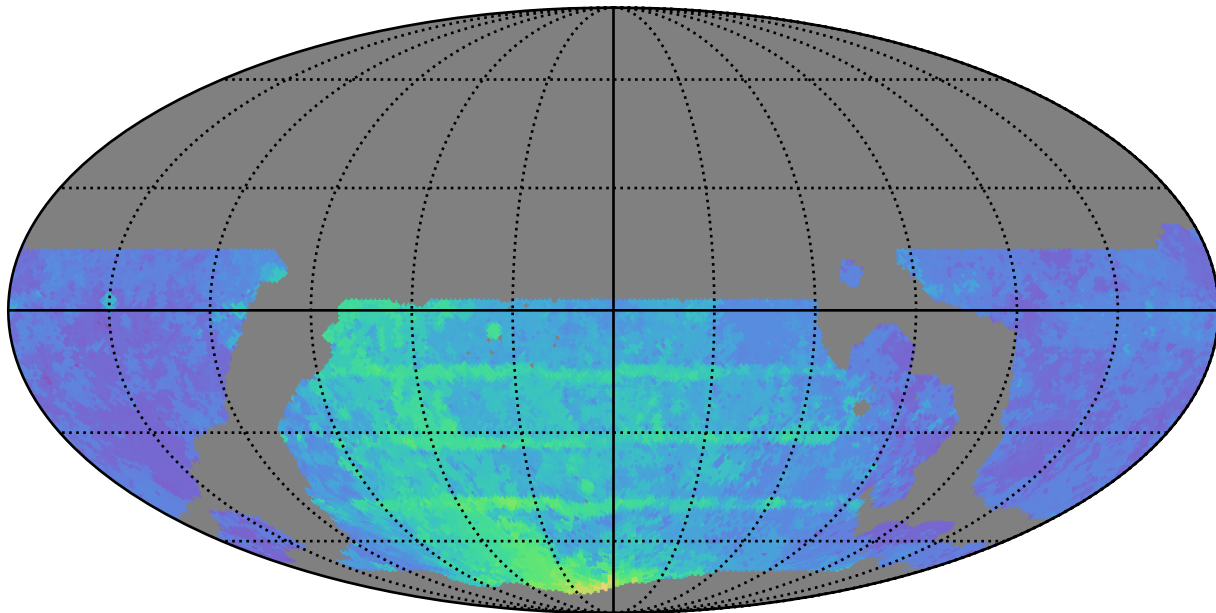
weather_cloudso36v3.4_10yrs WFD y band: 80thPercentile Season Length
