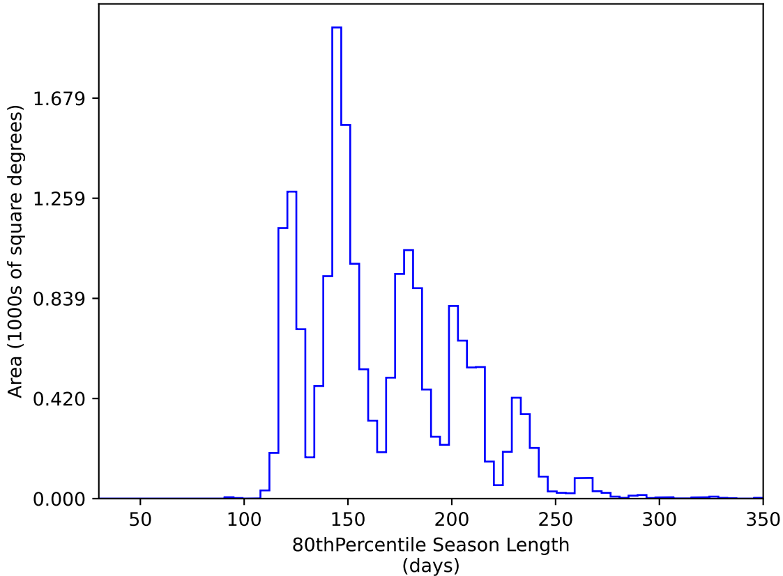
weather_cloudso36v3.4_10yrs WFD y band: 80thPercentile Season Length
