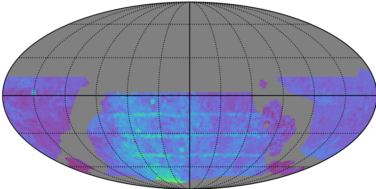
weather_cloudso36v3.4_10yrs WFD u band: 80thPercentile Season Length
