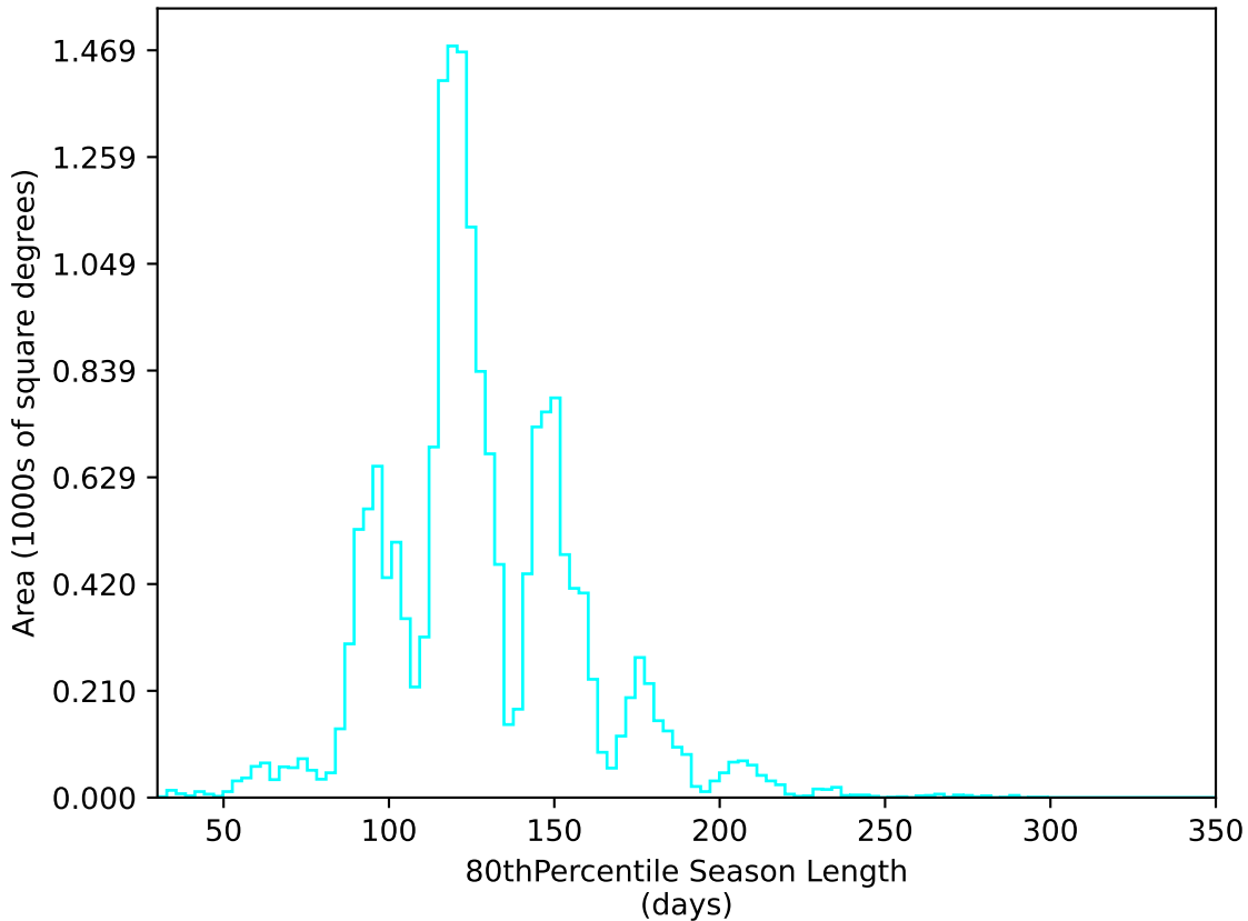
weather_cloudso36v3.4_10yrs WFD u band: 80thPercentile Season Length
