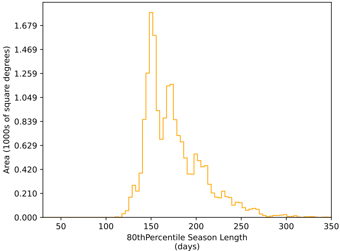
weather_cloudso36v3.4_10yrs WFD r band: 80thPercentile Season Length
