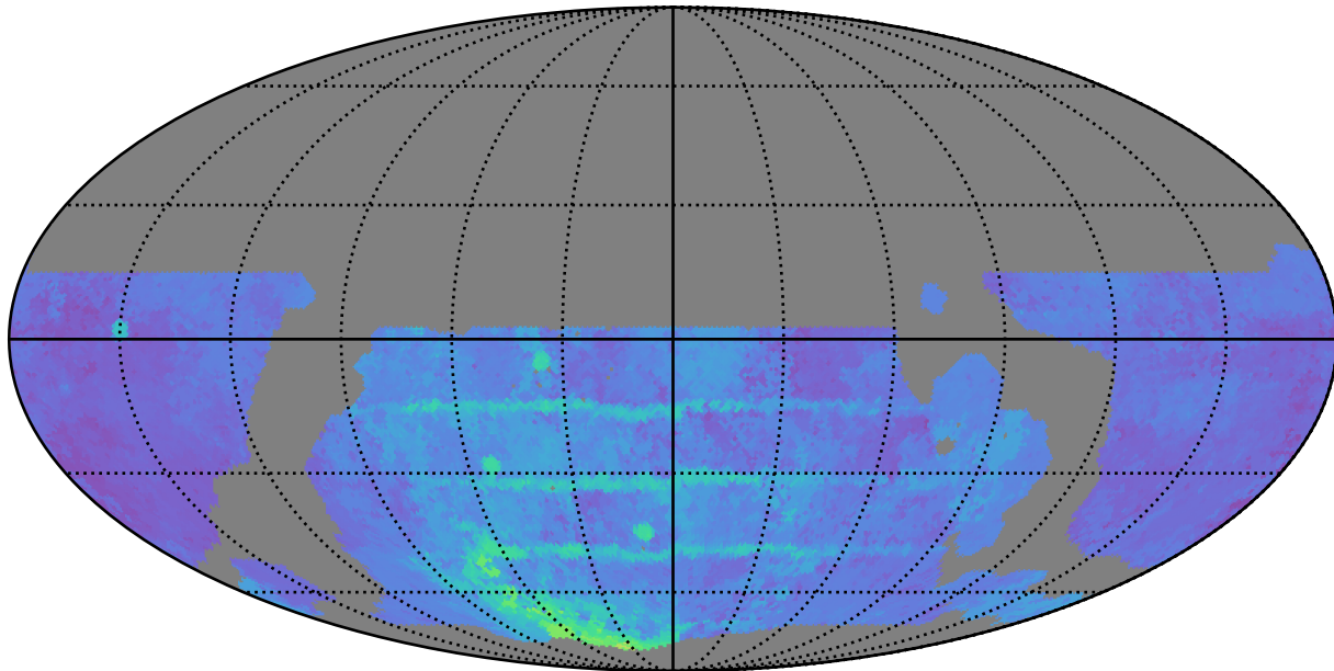
weather_cloudso36v3.4_10yrs WFD g band: 80thPercentile Season Length
