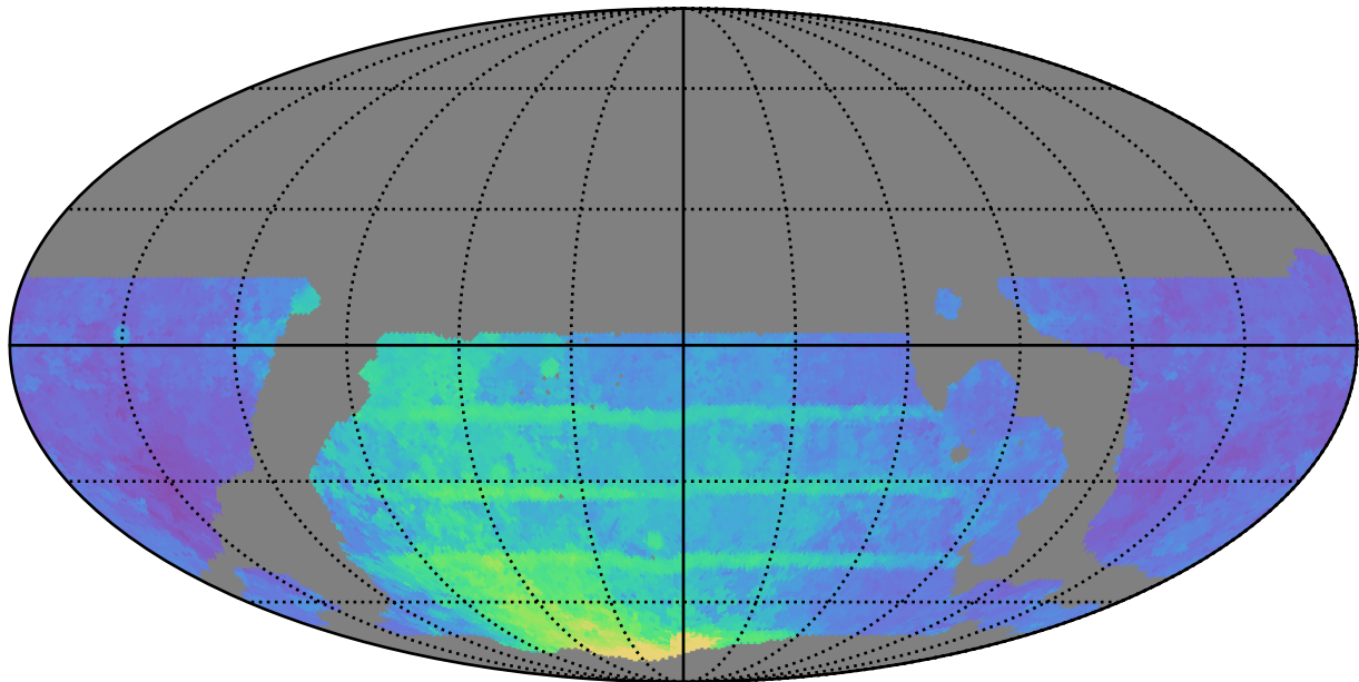
weather_cloudso36v3.4_10yrs WFD all bands: 80thPercentile Season Length
