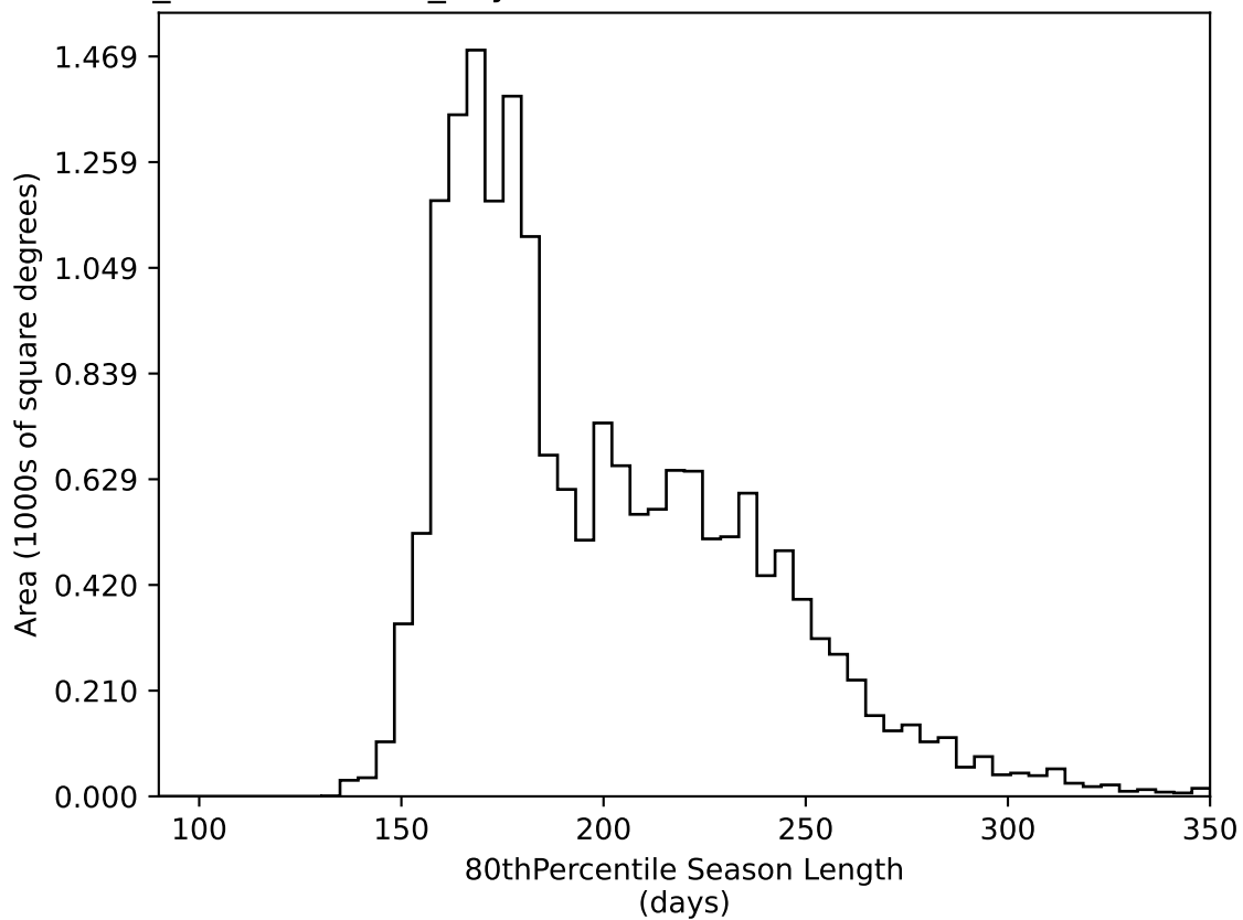
weather_cloudso36v3.4_10yrs WFD all bands: 80thPercentile Season Length
