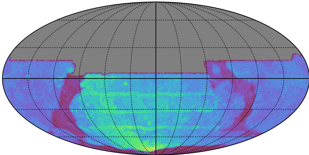
weather_cloudso36v3.4_10yrs All sky y band: 80thPercentile Season Length
