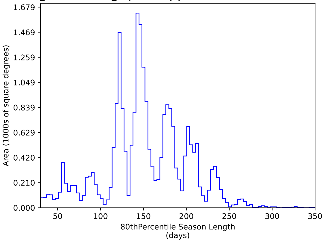
weather_cloudso36v3.4_10yrs All sky y band: 80thPercentile Season Length
