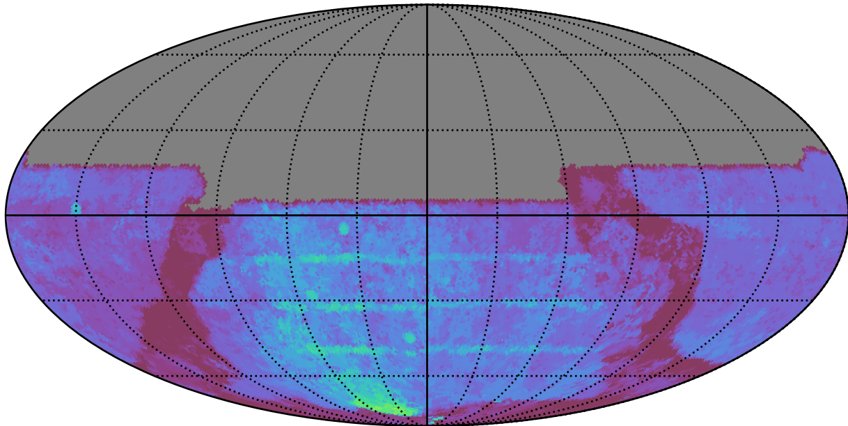
weather_cloudso36v3.4_10yrs All sky u band: 80thPercentile Season Length
