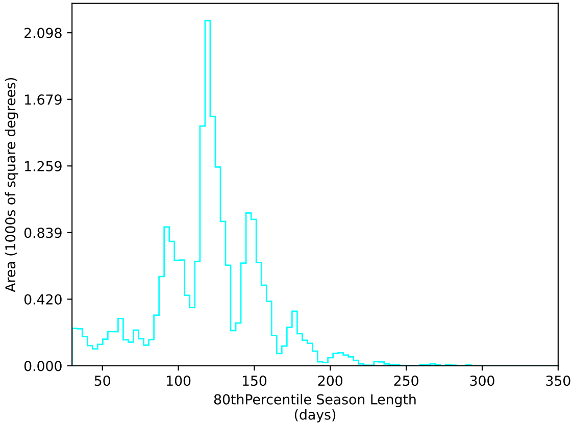
weather_cloudso36v3.4_10yrs All sky u band: 80thPercentile Season Length
