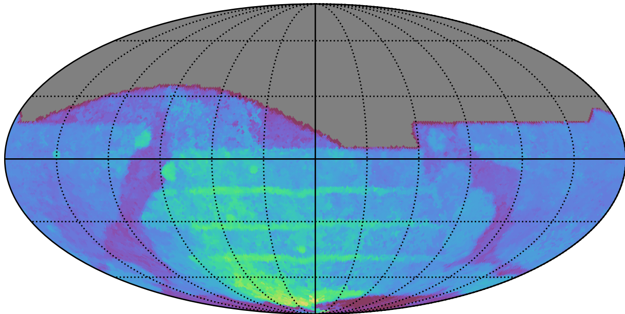
weather_cloudso36v3.4_10yrs All sky r band: 80thPercentile Season Length
