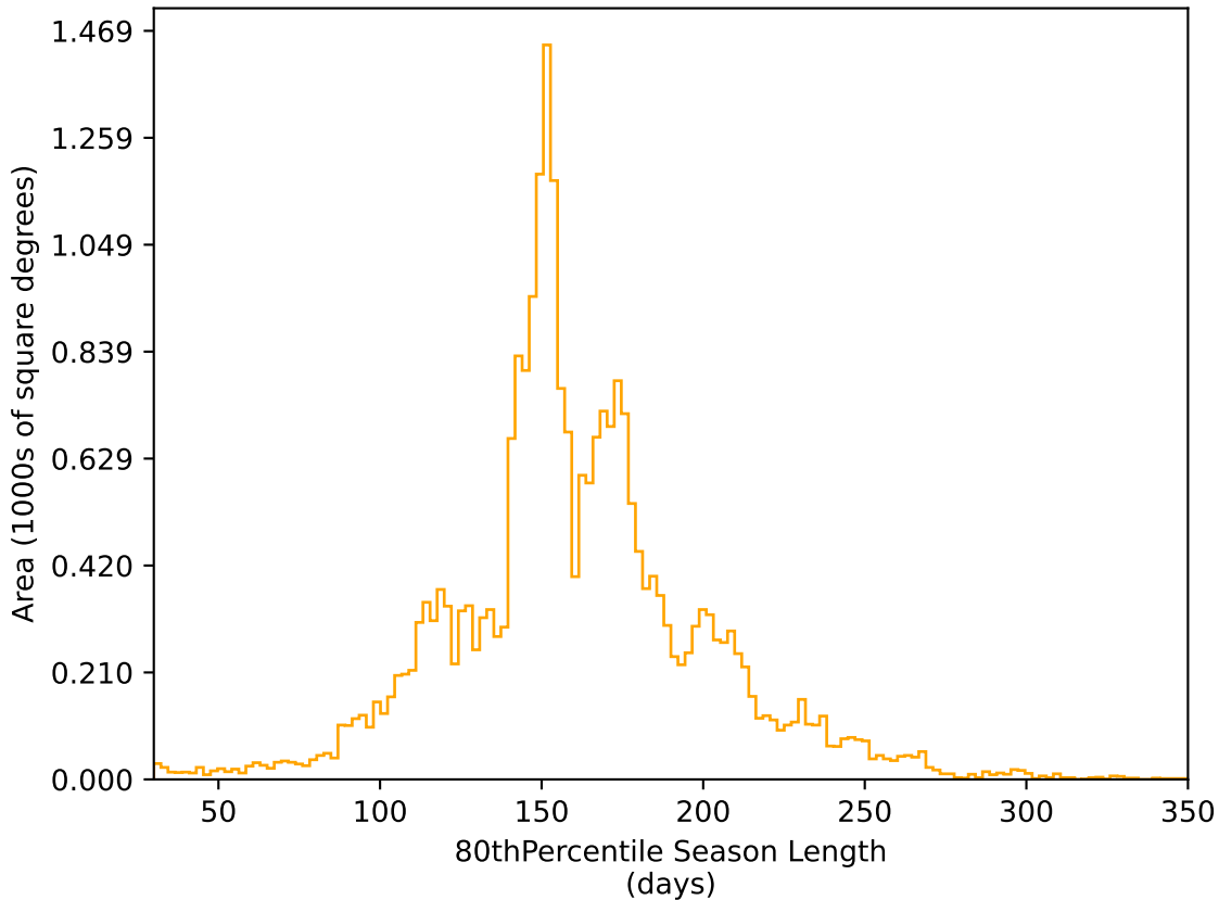
weather_cloudso36v3.4_10yrs All sky r band: 80thPercentile Season Length
