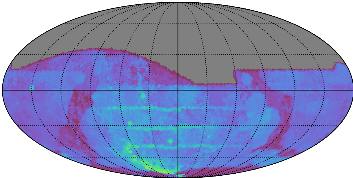
weather_cloudso36v3.4_10yrs All sky g band: 80thPercentile Season Length
