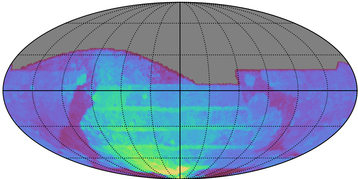
weather_cloudso36v3.4_10yrs All sky all bands: 80thPercentile Season Length
