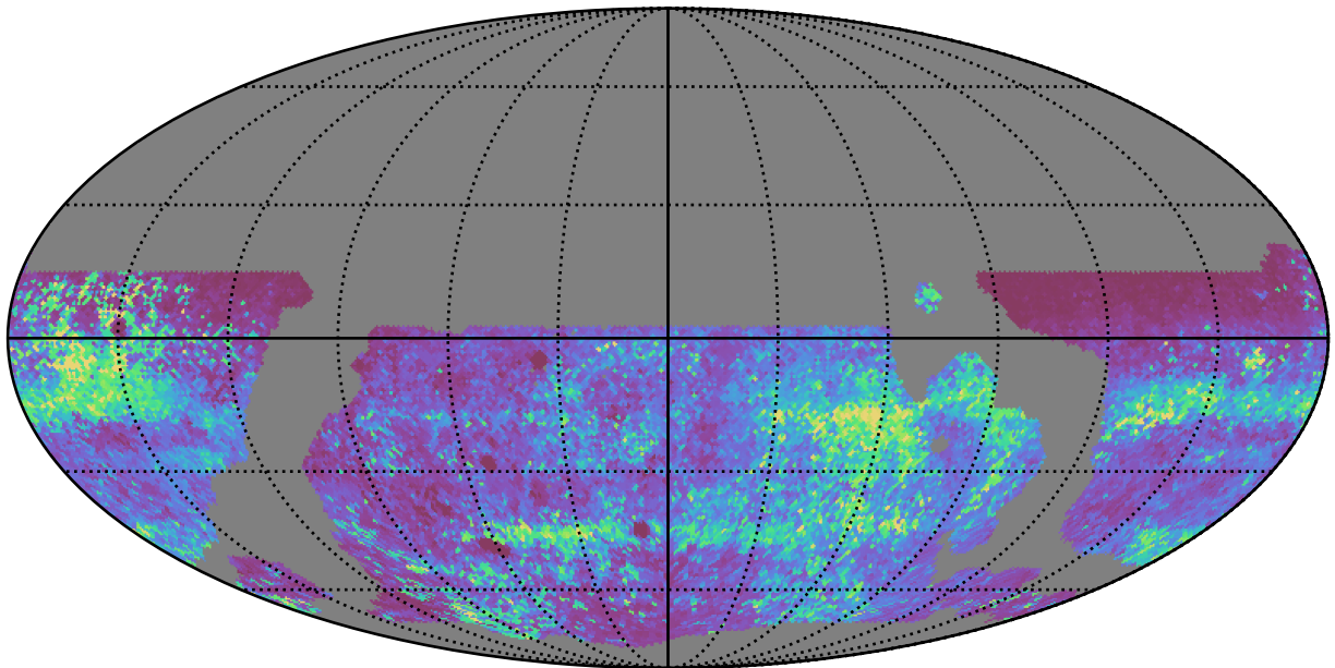
weather_cloudso36v3.4_10yrs WFD zy bands: 75th Percentile Intranight Timespan
