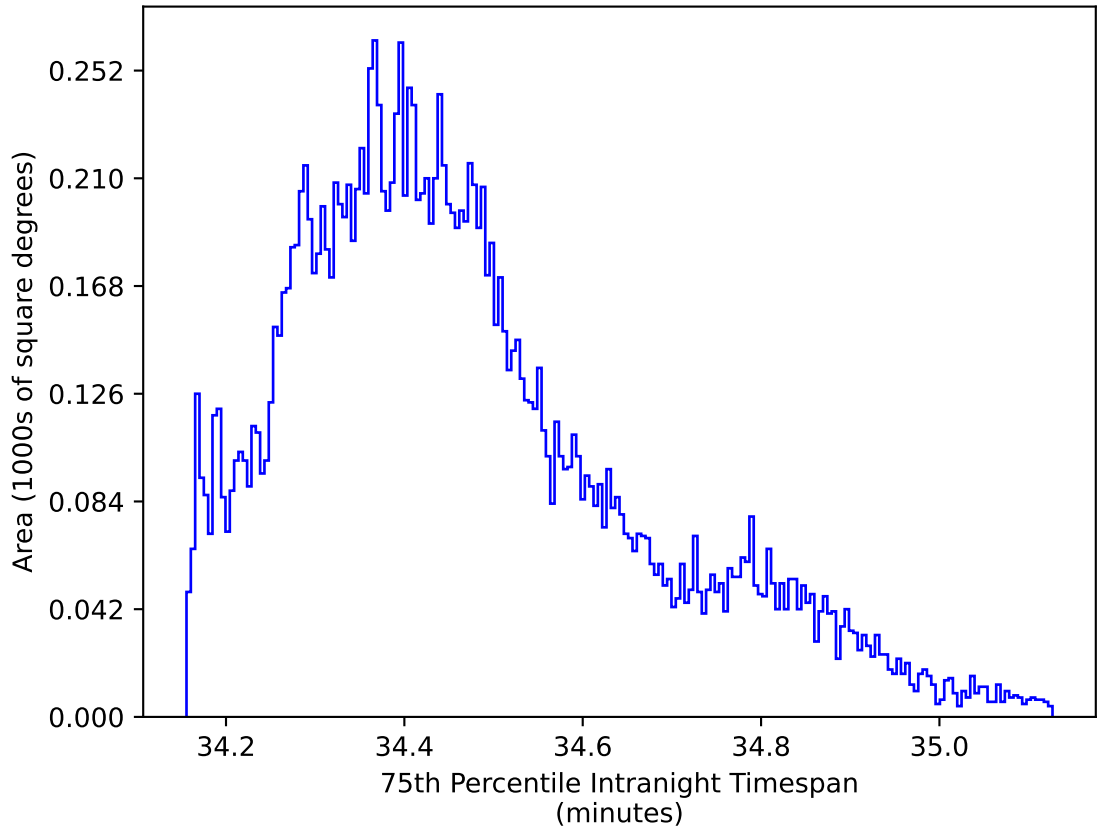
weather_cloudso36v3.4_10yrs WFD zy bands: 75th Percentile Intranight Timespan
