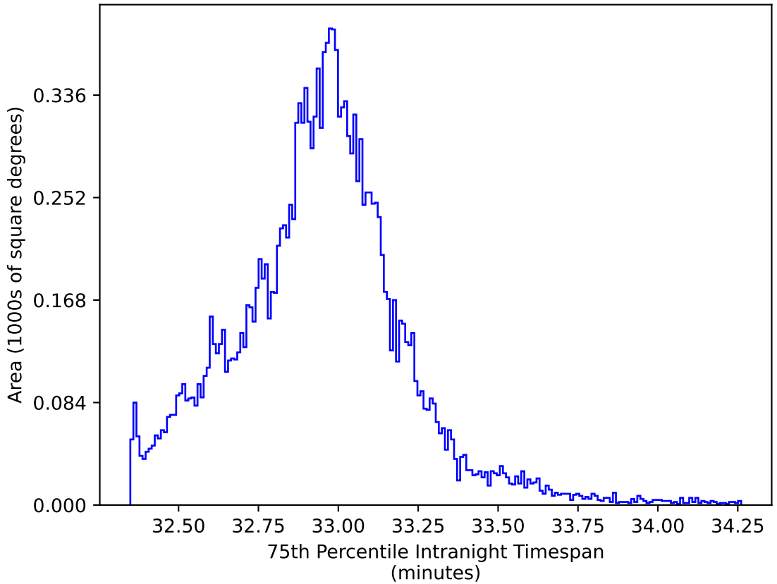
weather_cloudso36v3.4_10yrs WFD y band: 75th Percentile Intranight Timespan
