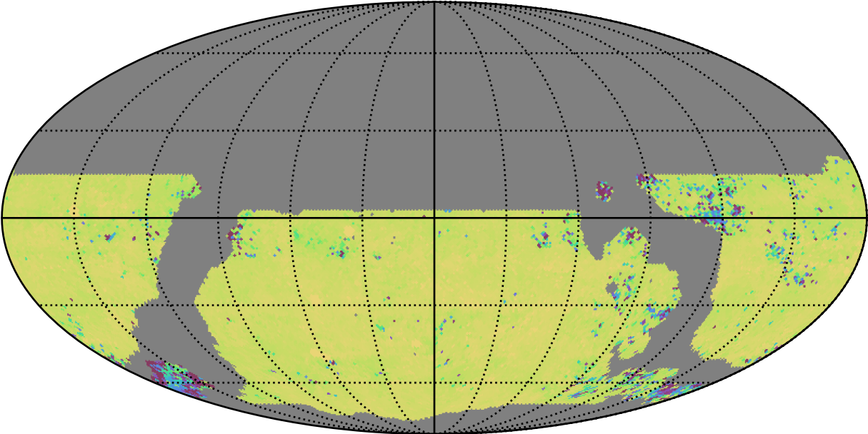
weather_cloudso36v3.4_10yrs WFD ug bands: 75th Percentile Intranight Timespan
