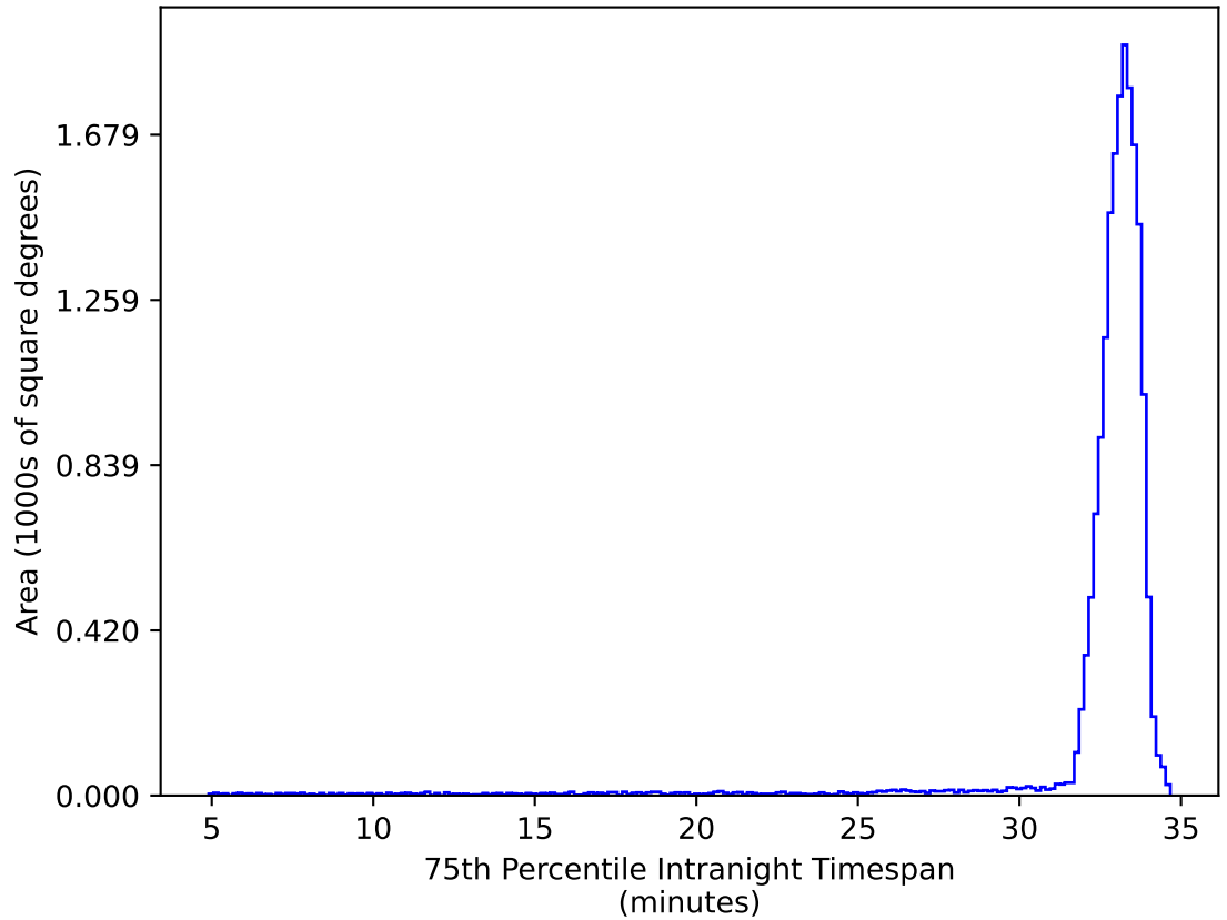
weather_cloudso36v3.4_10yrs WFD ug bands: 75th Percentile Intranight Timespan
