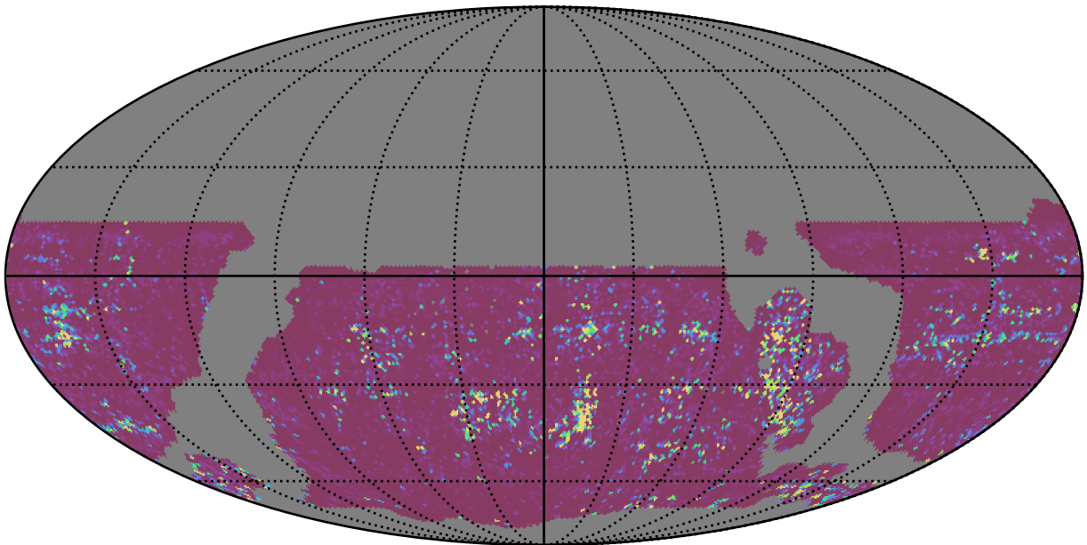
weather_cloudso36v3.4_10yrs WFD u band: 75th Percentile Intranight Timespan
