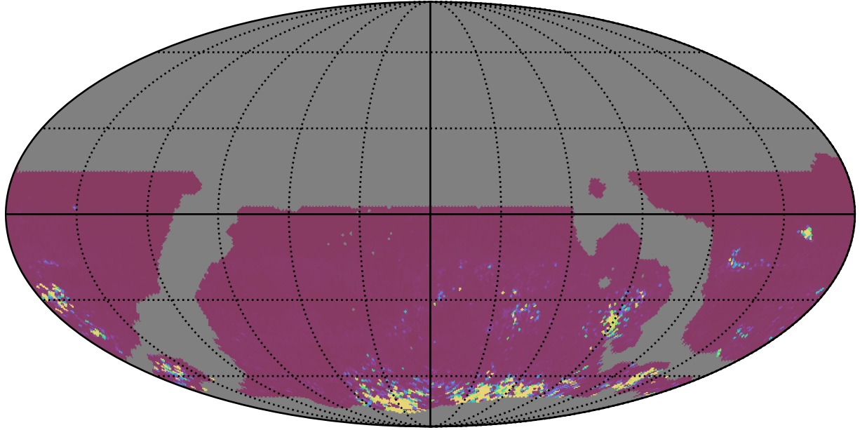
weather_cloudso36v3.4_10yrs WFD ri bands: 75th Percentile Intranight Timespan
