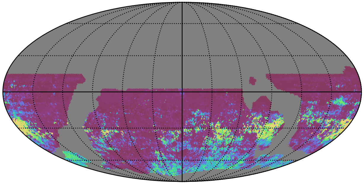
weather_cloudso36v3.4_10yrs WFD r band: 75th Percentile Intranight Timespan
