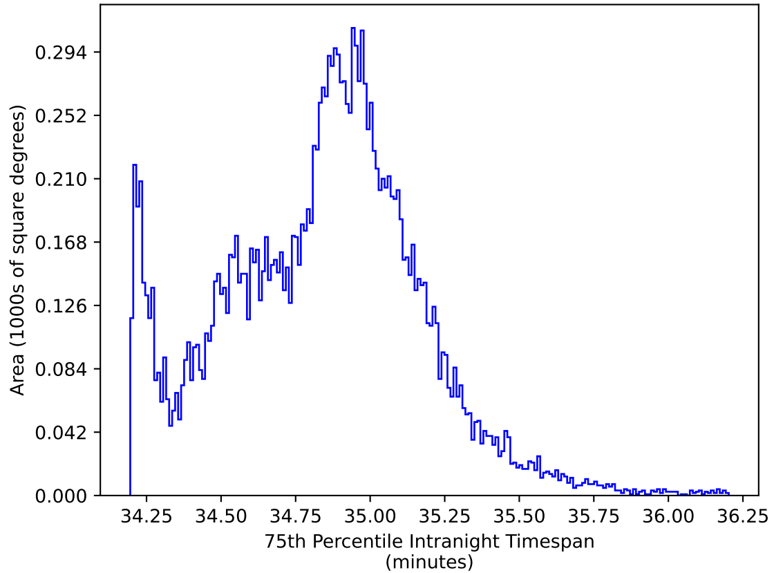
weather_cloudso36v3.4_10yrs WFD iz bands: 75th Percentile Intranight Timespan
