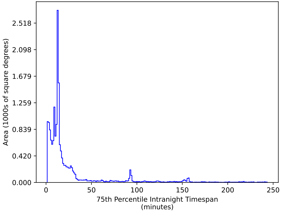
weather_cloudso36v3.4_10yrs WFD i band: 75th Percentile Intranight Timespan
