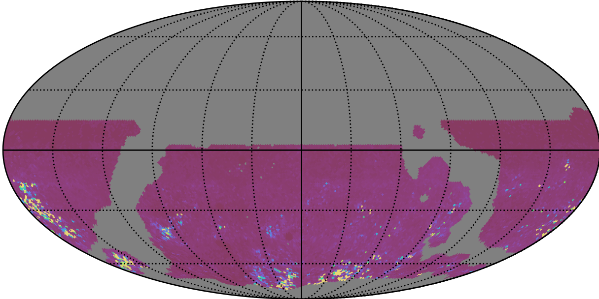
weather_cloudso36v3.4_10yrs WFD gr bands: 75th Percentile Intranight Timespan
