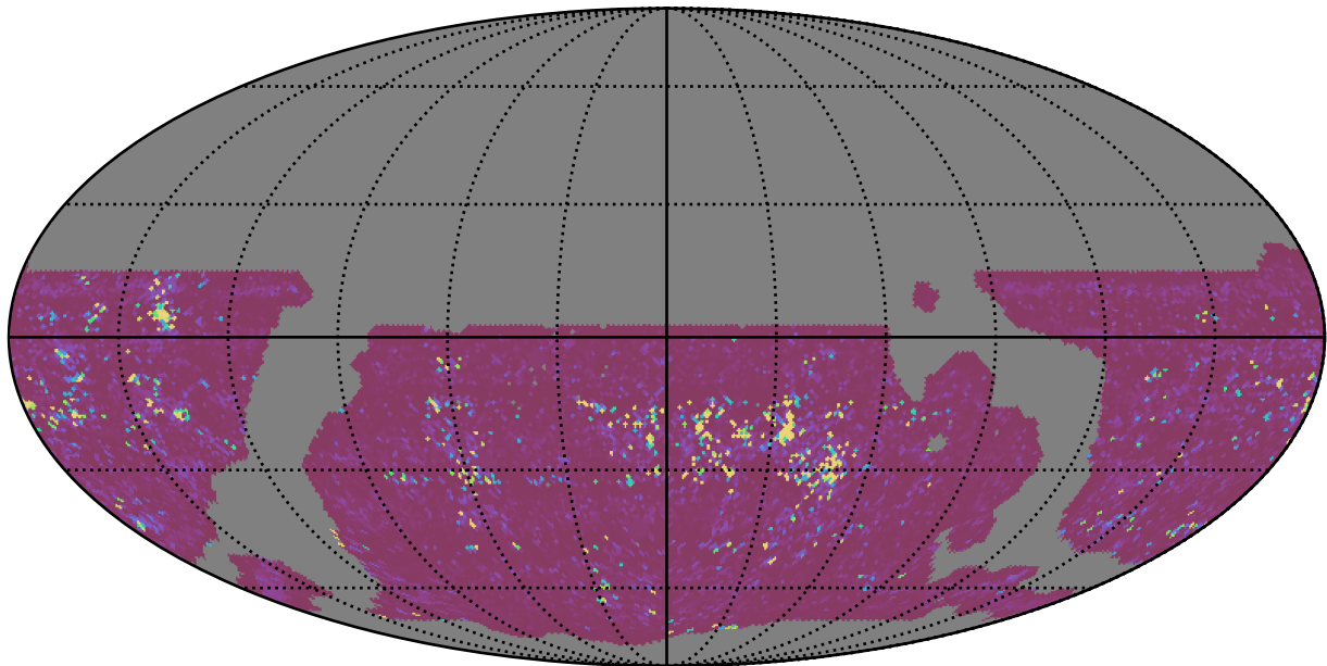
weather_cloudso36v3.4_10yrs WFD g band: 75th Percentile Intranight Timespan
