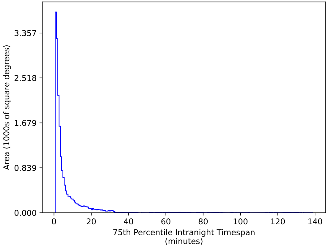
weather_cloudso36v3.4_10yrs WFD g band: 75th Percentile Intranight Timespan
