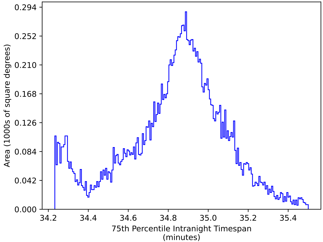
weather_cloudso36v3.4_10yrs WFD all bands: 75th Percentile Intranight Timespan
