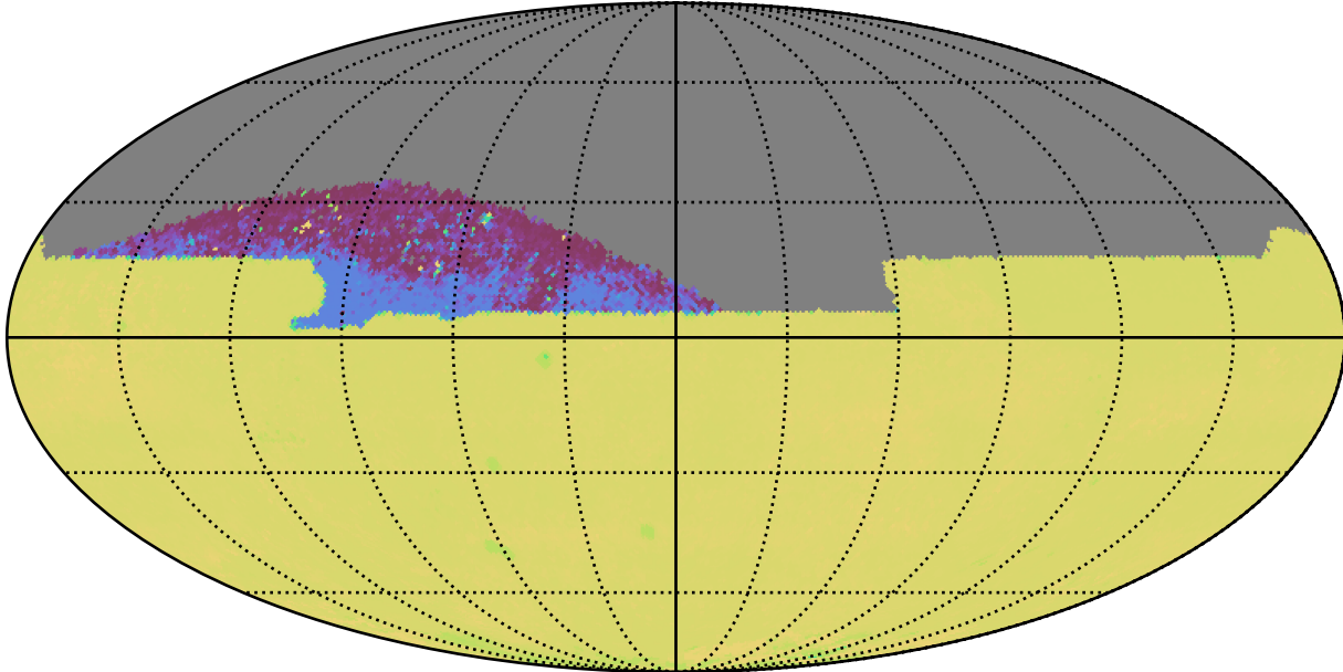
weather_cloudso36v3.4_10yrs All sky zy bands: 75th Percentile Intranight Timespan
