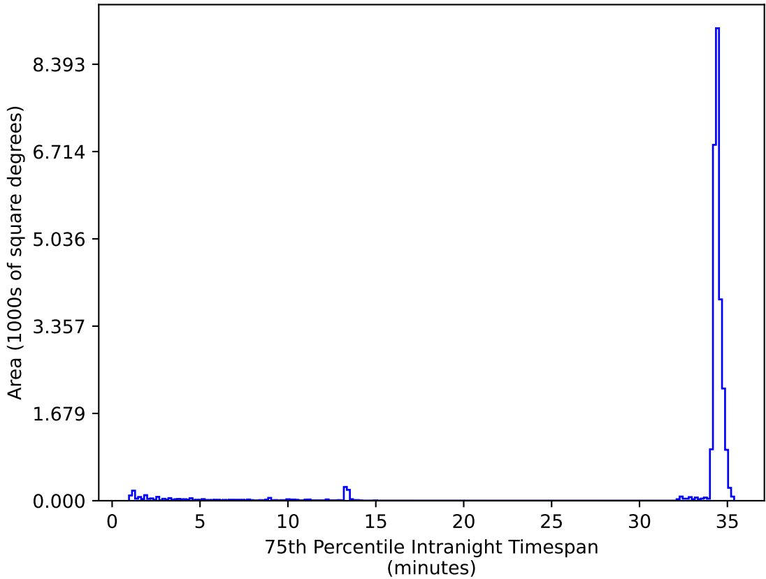
weather_cloudso36v3.4_10yrs All sky zy bands: 75th Percentile Intranight Timespan
