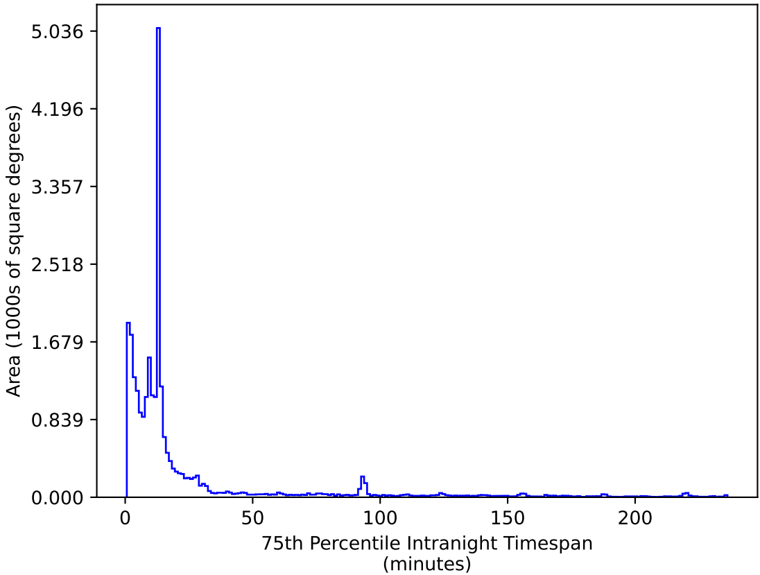
weather_cloudso36v3.4_10yrs All sky z band: 75th Percentile Intranight Timespan
