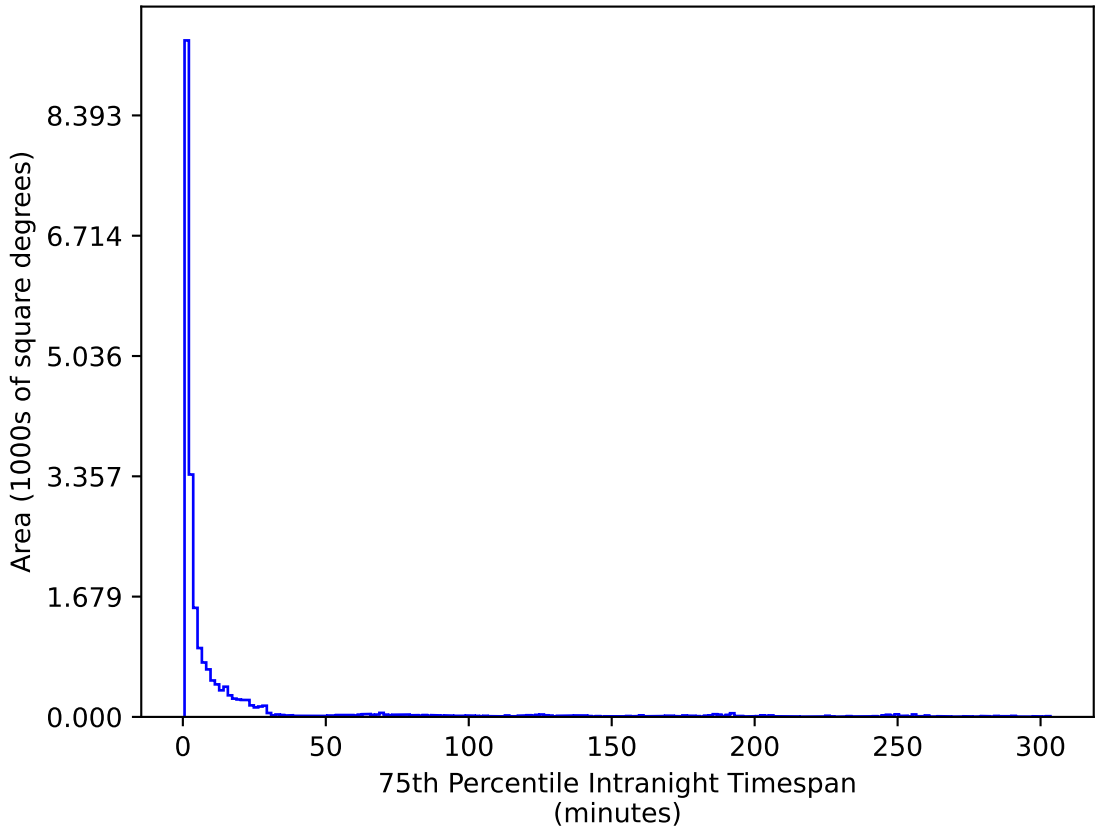
weather_cloudso36v3.4_10yrs All sky u band: 75th Percentile Intranight Timespan
