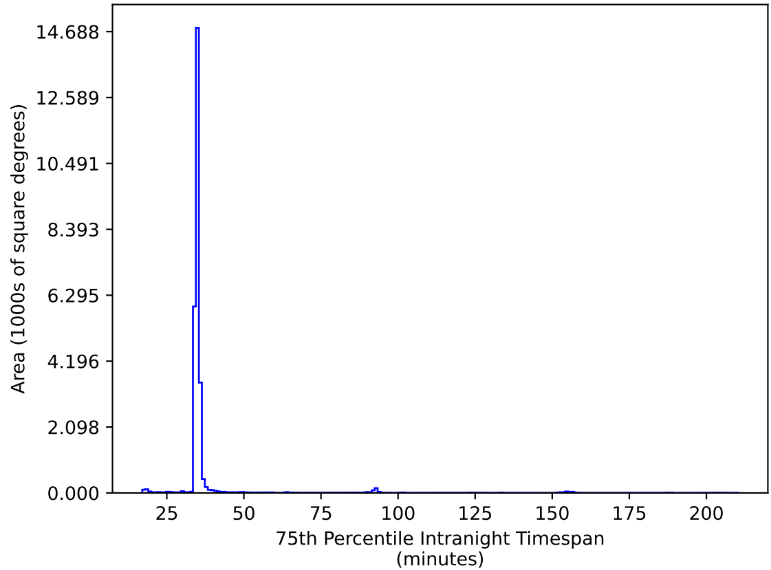
weather_cloudso36v3.4_10yrs All sky ri bands: 75th Percentile Intranight Timespan
