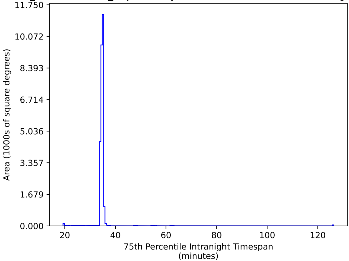
weather_cloudso36v3.4_10yrs All sky iz bands: 75th Percentile Intranight Timespan
