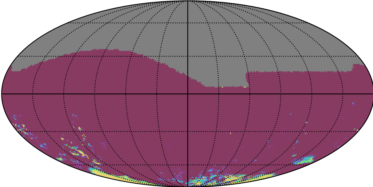
weather_cloudso36v3.4_10yrs All sky gr bands: 75th Percentile Intranight Timespan
