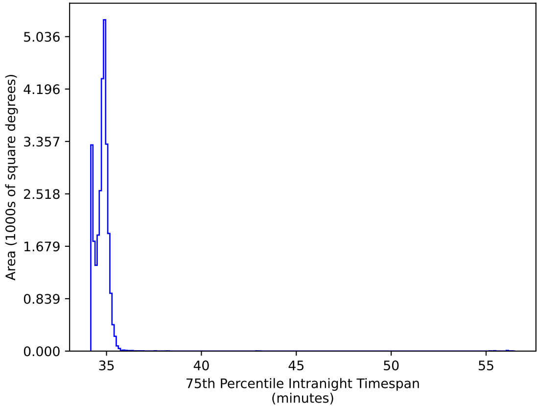
weather_cloudso36v3.4_10yrs All sky all bands: 75th Percentile Intranight Timespan
