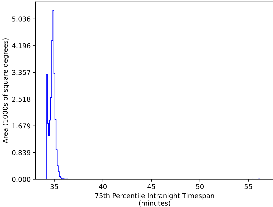
weather_cloudso36v3.4_10yrs All sky: 75th Percentile Intranight Timespan
