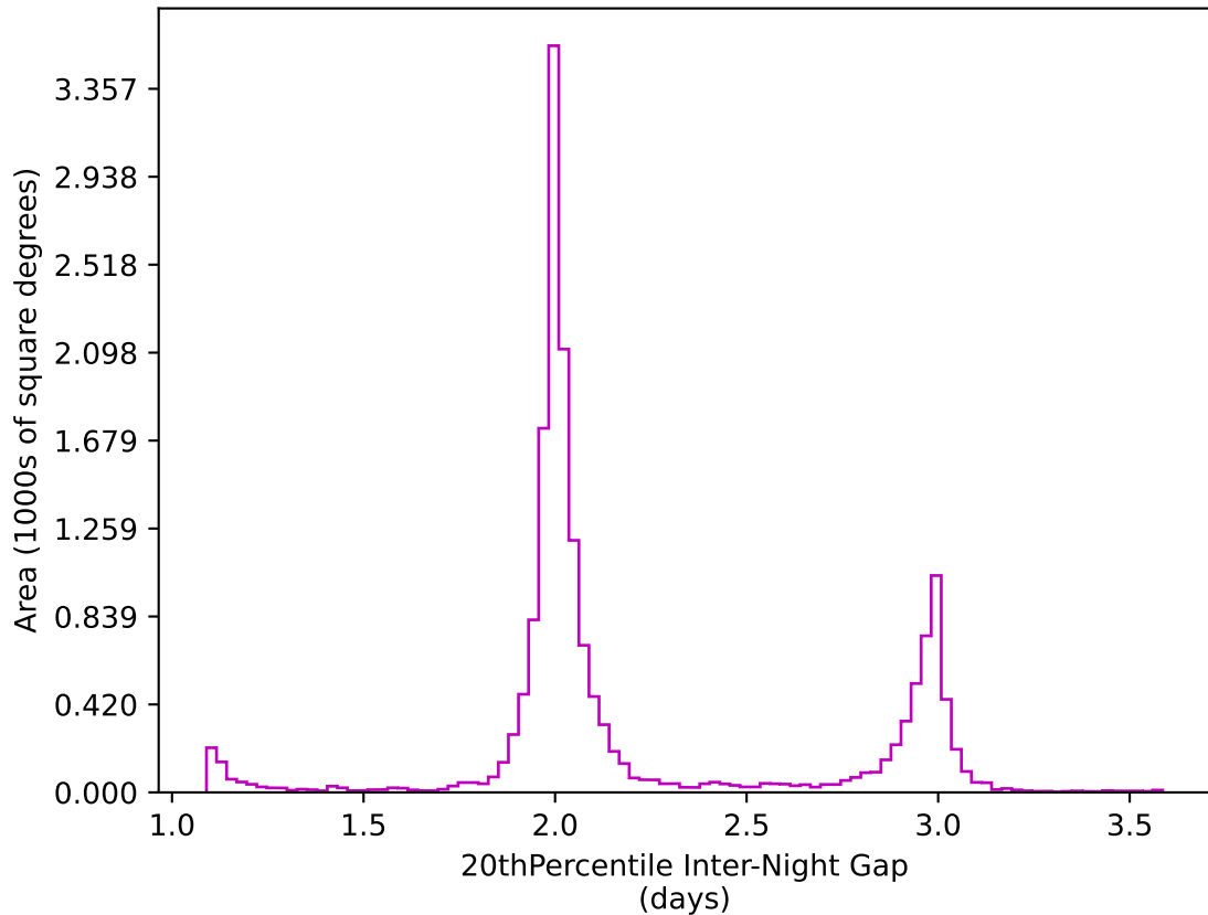
weather_cloudso36v3.4_10yrs WFD z band: 20thPercentile Inter-Night Gap
