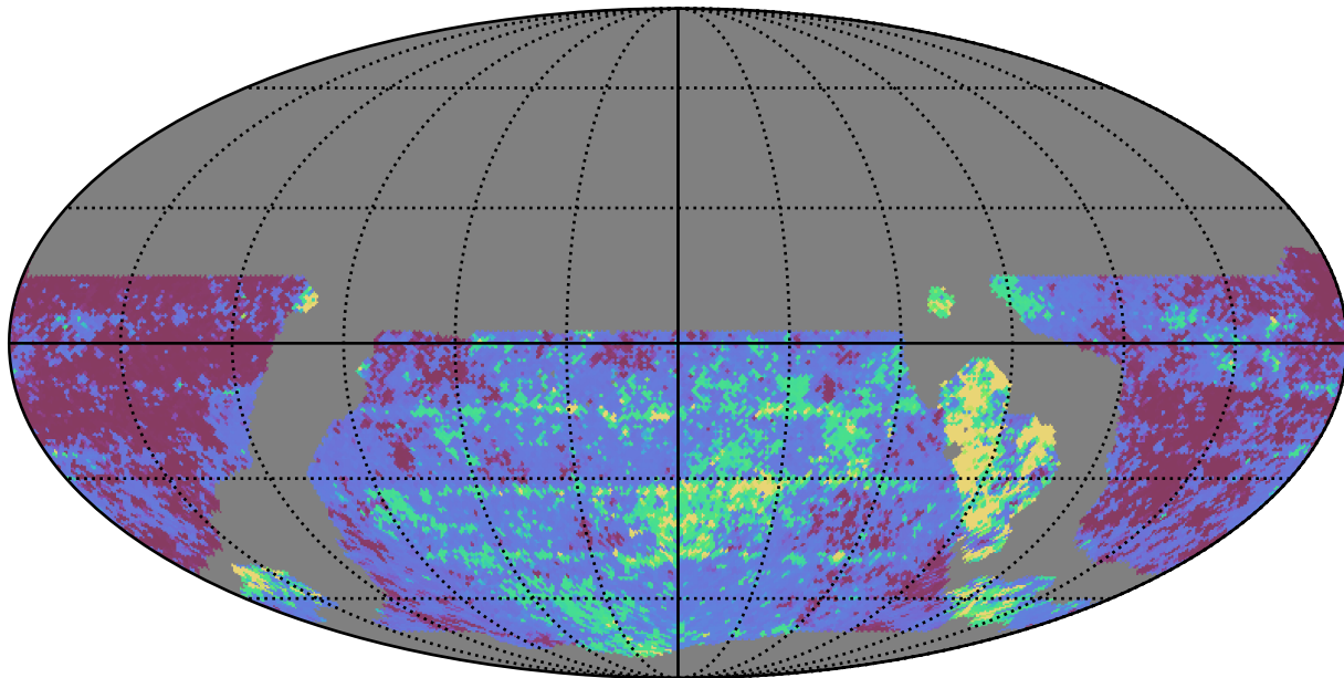
weather_cloudso36v3.4_10yrs WFD y band: 20thPercentile Inter-Night Gap
