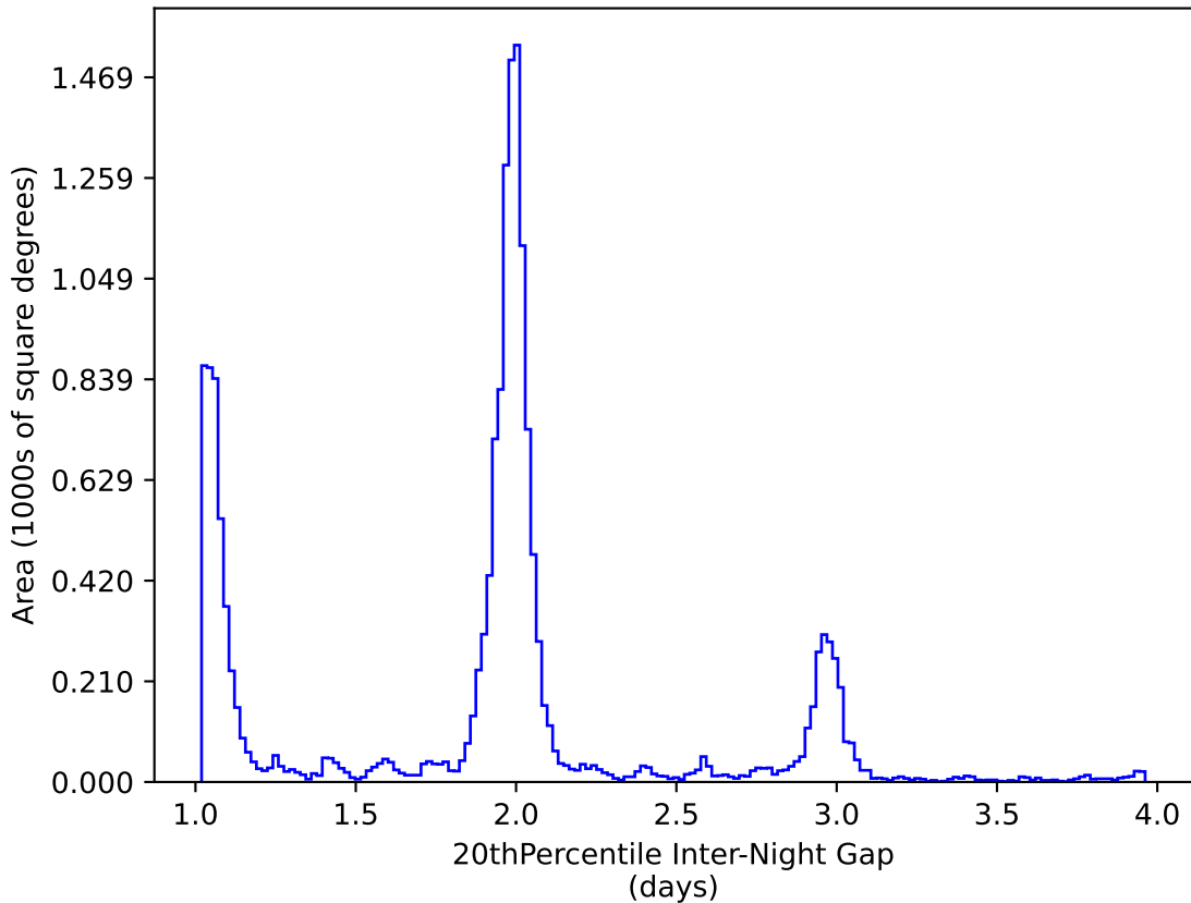
weather_cloudso36v3.4_10yrs WFD y band: 20thPercentile Inter-Night Gap
