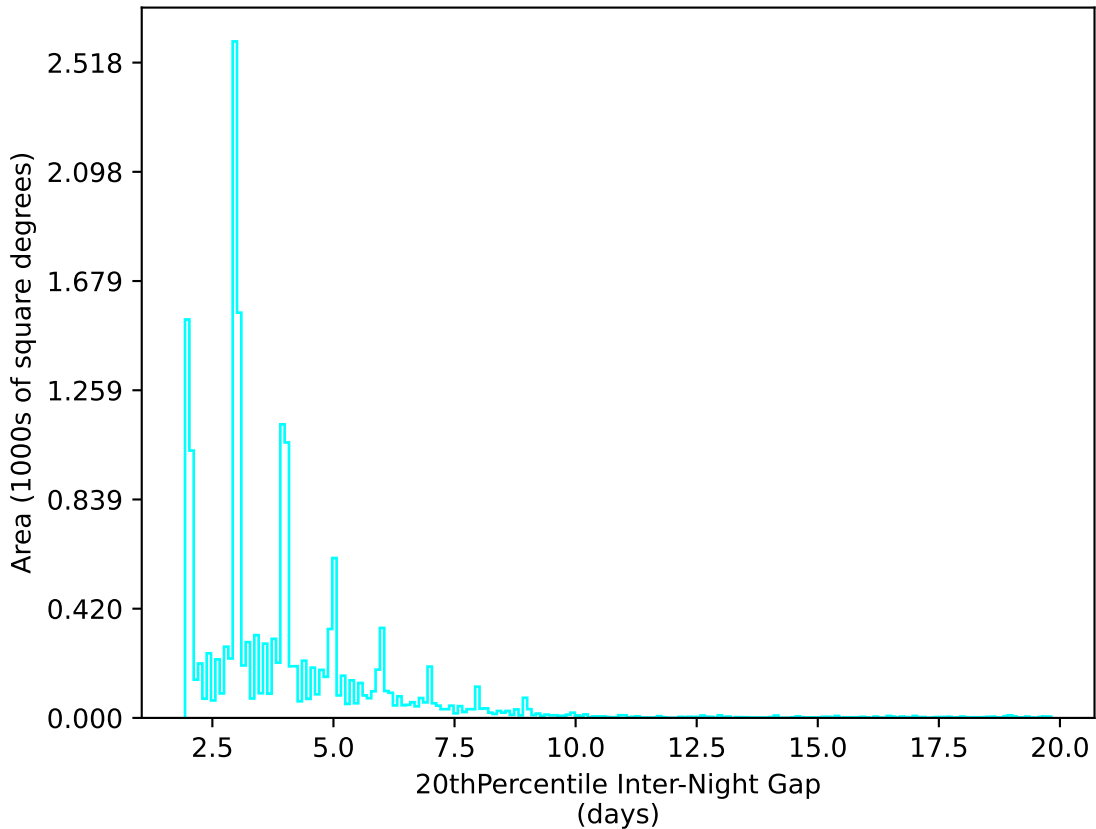
weather_cloudso36v3.4_10yrs WFD u band: 20thPercentile Inter-Night Gap
