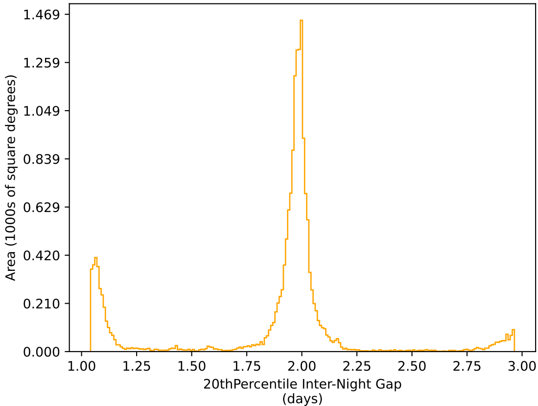
weather_cloudso36v3.4_10yrs WFD r band: 20thPercentile Inter-Night Gap
